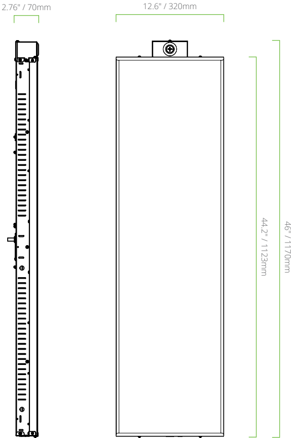
MODELS: LHS1-PS240W - 320W 240W Weight: 13.5 lbs / 6.13 kg 320W Weight: 14.6 lbs / 6.62 kg Master Carton Weight: 17.6 lbs Dimensions: 47.05" x 4.13" 13.58"
